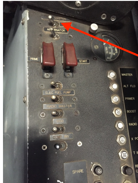
Cockpit Forward Lower Right Side
